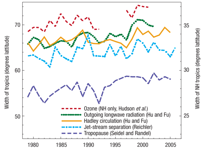
Figure 2 Changes in several estimates of the width of the tropical belt since 1979. These include: the width of the Hadley circulation, based on both outgoing longwave radiation and horizontal winds streamfunction 9 ; the separation of the Northern and Southern Hemisphere subtropical jet-stream cores; the width of the region of frequent high tropopause levels 8 ; and the width of the region with tropical column ozone levels (Northern Hemisphere only, right axis, ref. 6). Although each shows an increase since 1979, the rates vary from 2.0 to 4.8 degrees latitude per 25 years, with an even larger range when considering the entire spread of trend estimates in each individual study.
